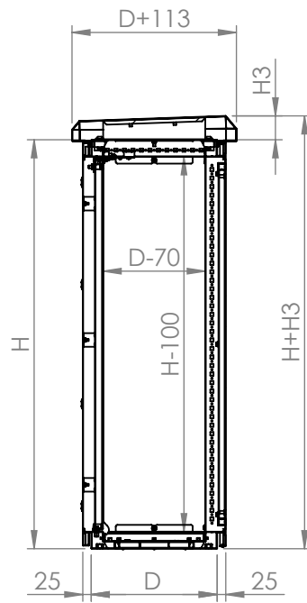
SECTION X-X
