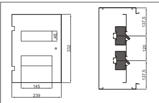
Enclosure W300 x H400 mm Product Code: 943.856
