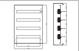
Enclosure W600 x H800 mm Product Code: 943.862
