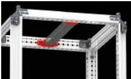
Combination on the top frame
