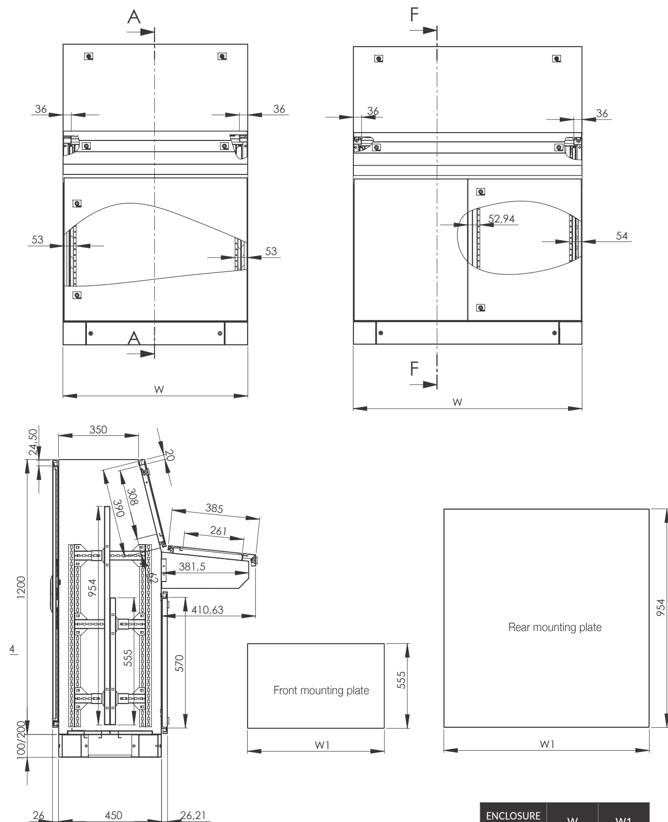
SECTION F-F SCALE 1 : 10
