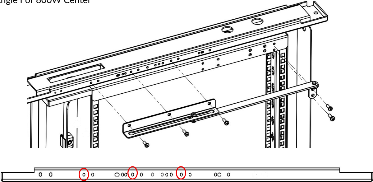
180 Angle For 800W Center
