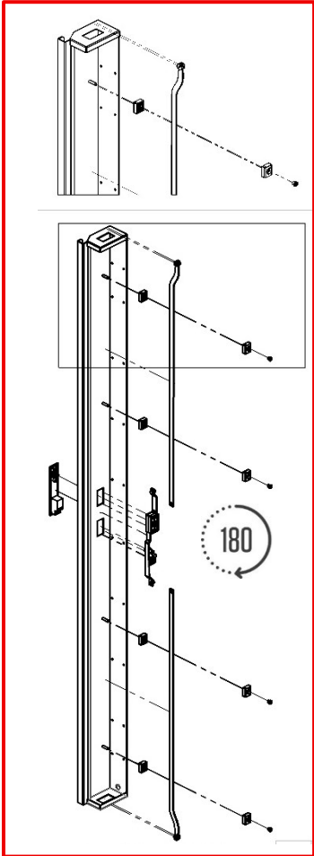
Lock Disassembly
