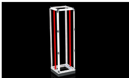
Vertical frame combination
