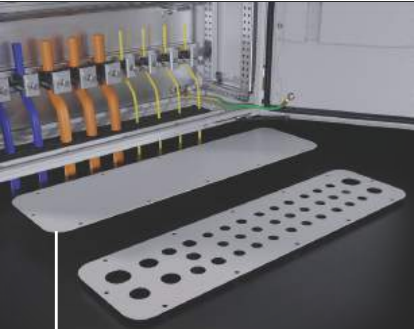
Gland plate structure with a flat and wide usage area and earthing integration. Safety and functionality with cable management options. Earthing integration
