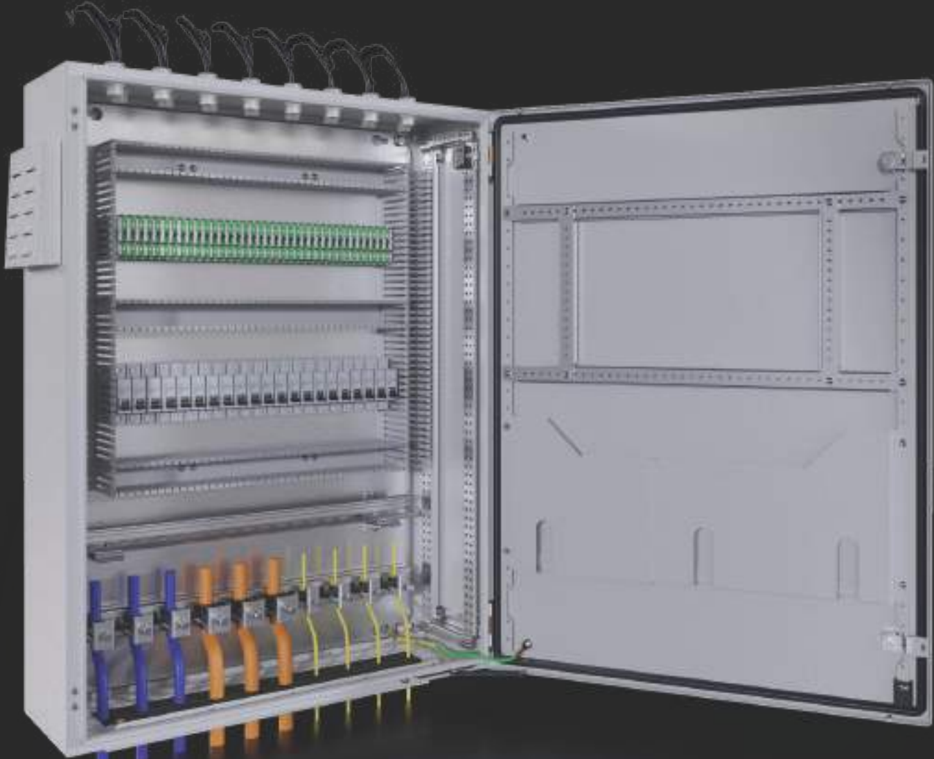
Large interior volume and wide door applications with thin curved body structure
