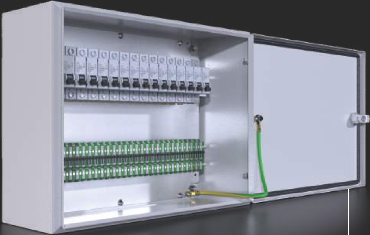
Earthing integration easy access with 180° opening hinge
