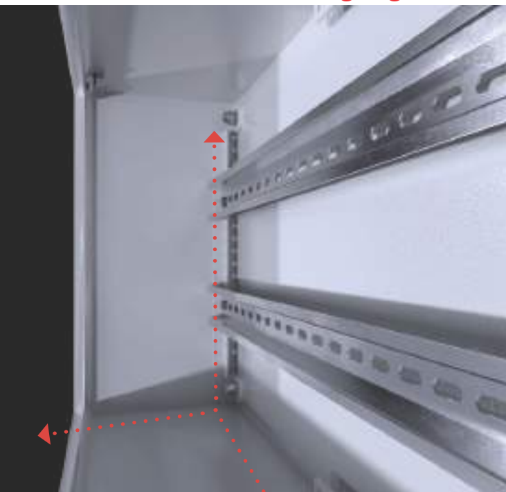
Mountable with 7.5 - 15 mm DIN rail for wide usage area Possibility to attach mounting plate with wide usage area
