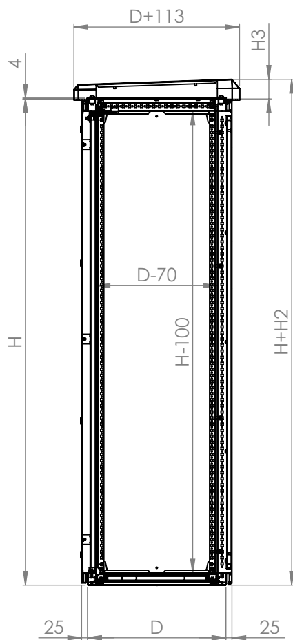
SECTION X-X
