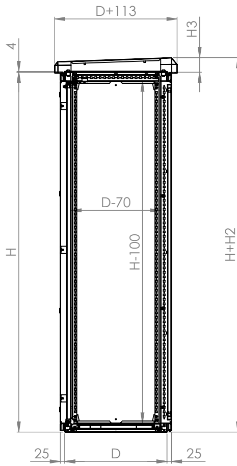
SECTION X-X
