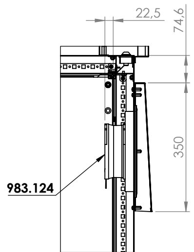
DETAIL A SCALE 1 : 10
